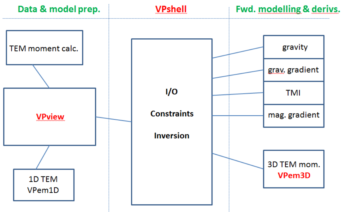
Figure 1.1: Schematic illustrating the structure of the “VP” software suite. VPem3D v2 is a specialised forward modelling module, linked to the VPshell which includes the inversion routines. VPview is the user interface.
