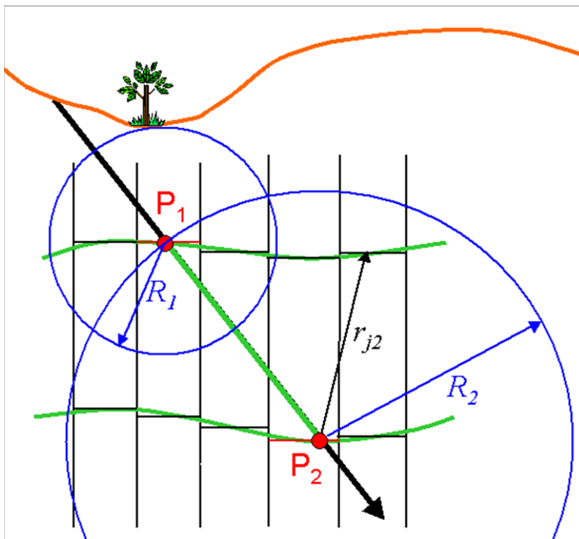
Figure 2.6: Movement of boundaries during geometry inversion is damped within a spherical volume centred on each fixed boundary.
