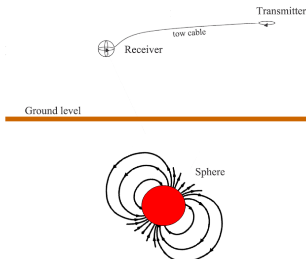
Figure 3.2: In the resistive limit, a conductive sphere produces a magnetic dipole response. This is the basis for the forward modelling algorithms in VPem3D.
